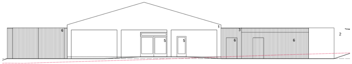
Proposed west elevation
